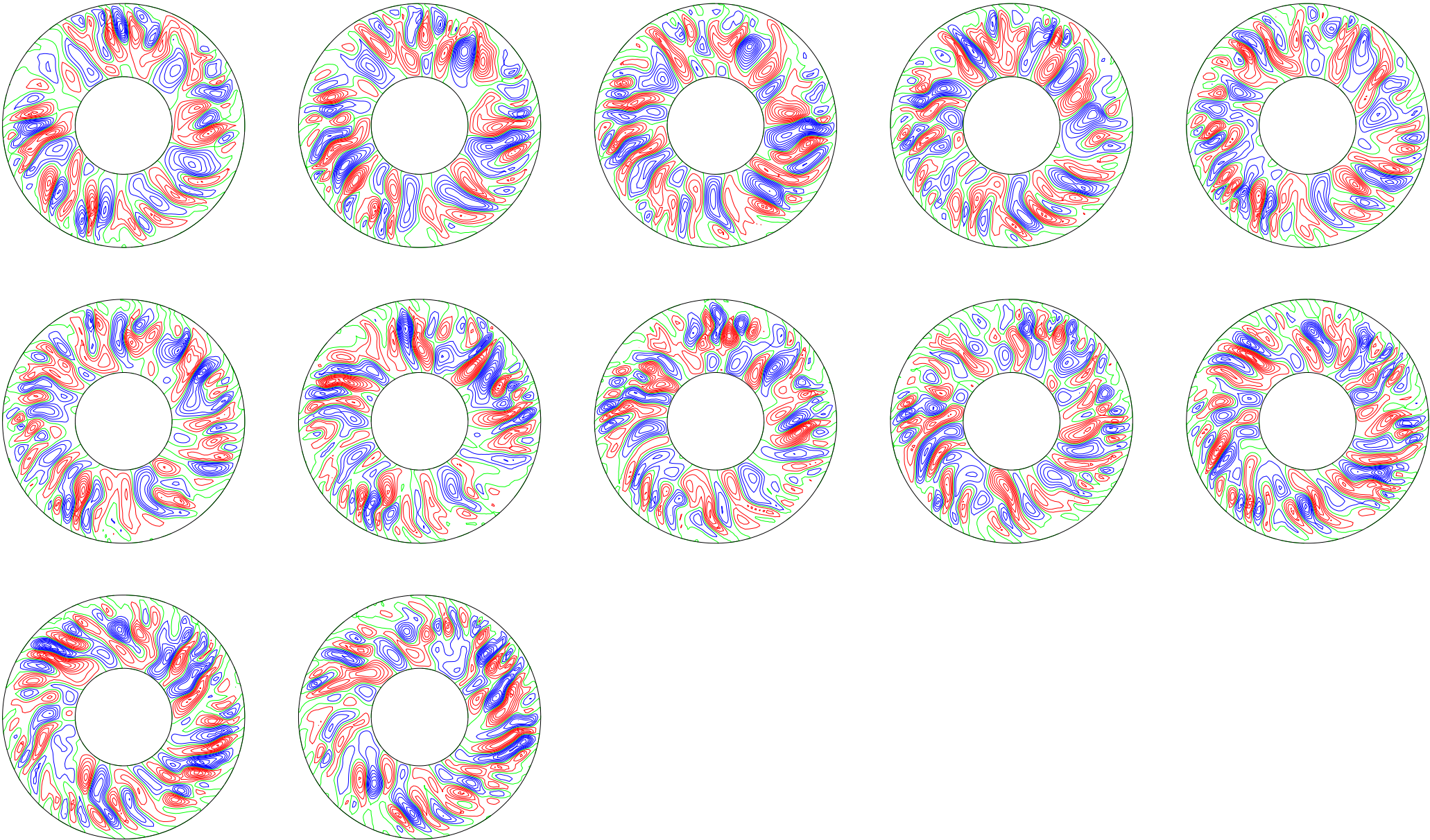
poloidal streamlines, (t[i] dt[i] t[i+1]): 2.14229 ( 0.003 ) 2.175301
