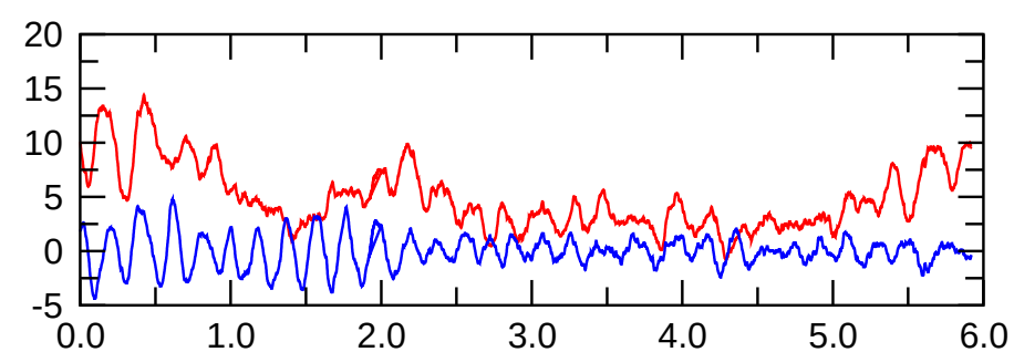
\text{pol}(m=0) magn.
