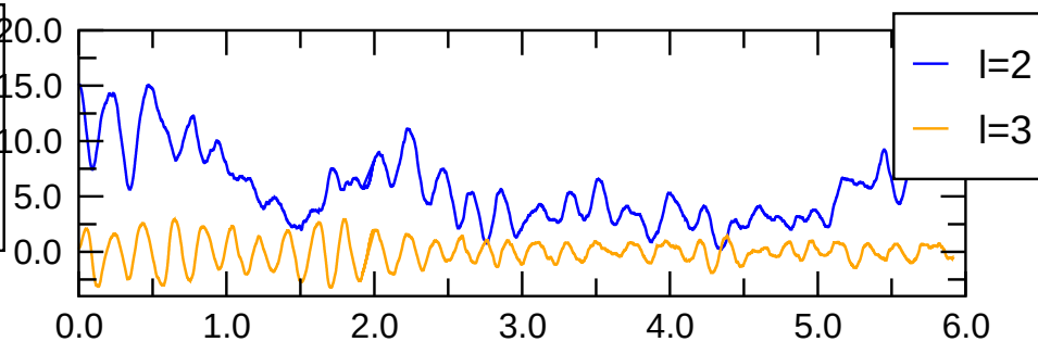
\text{pol}(m=0) magn.
