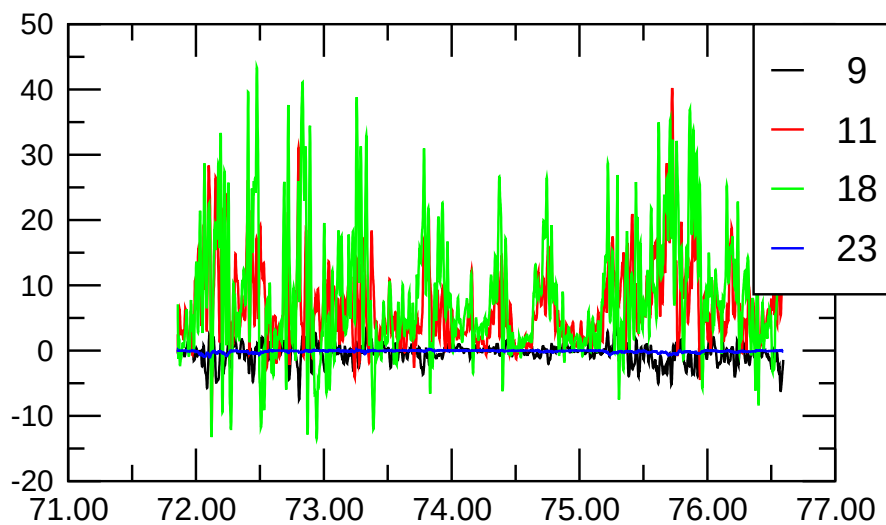
fluct-pol
