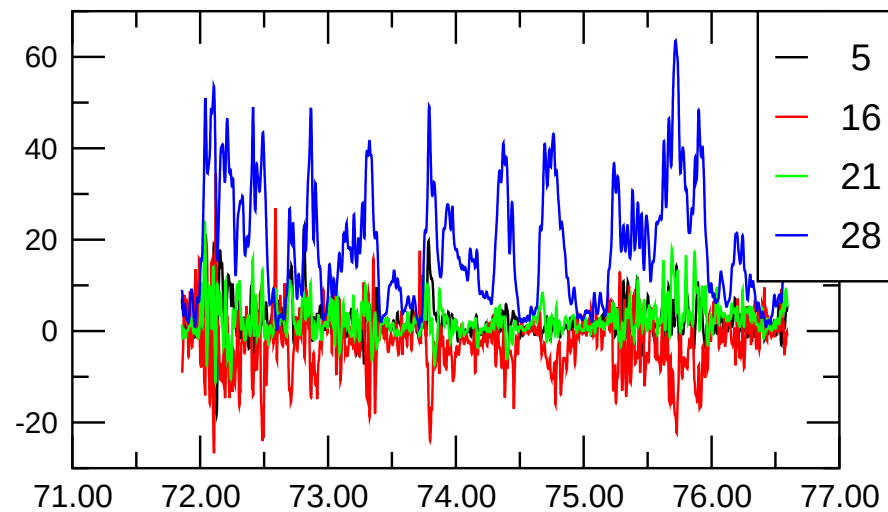
fluct-tor
