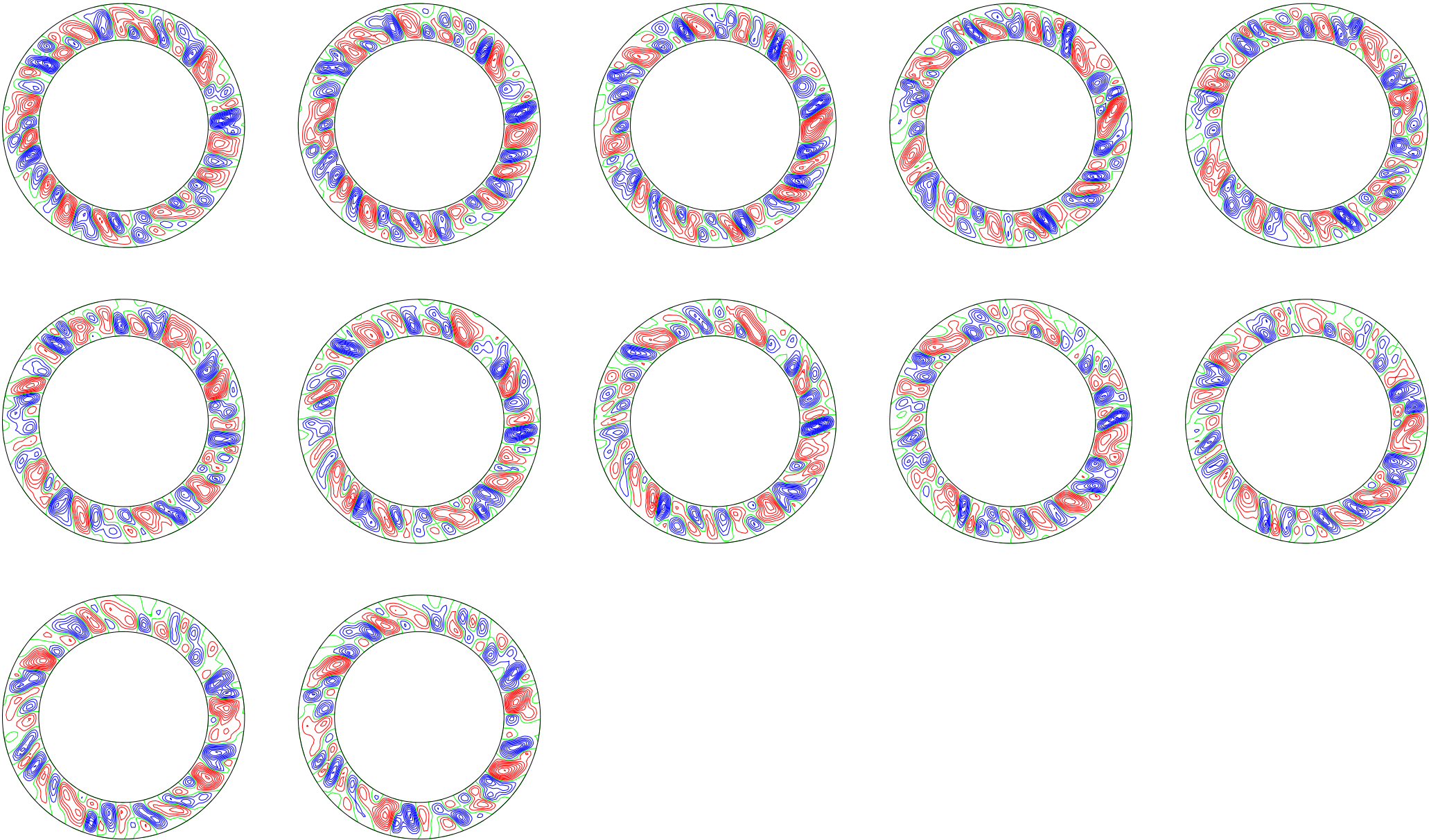
poloidal streamlines, (t[i] dt[i] t[i+1]): 74.81124 ( 0.007 ) 74.88835
