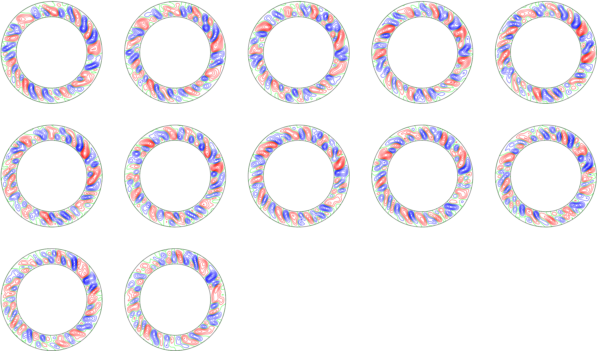
poloidal streamlines, (t[i] dt[i] t[i+1]): 75.23184 ( 0.007 ) 75.30895
