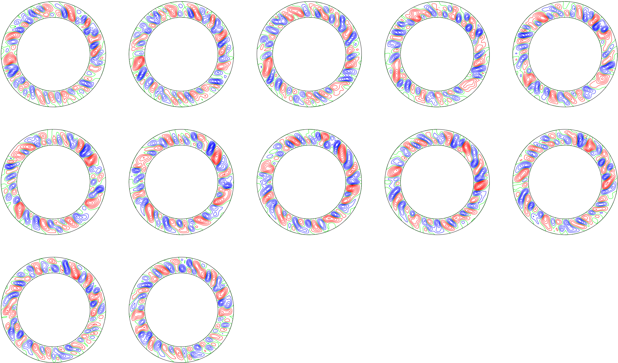
poloidal streamlines, (t[i] dt[i] t[i+1]): 75.40008 ( 0.007 ) 75.47719
