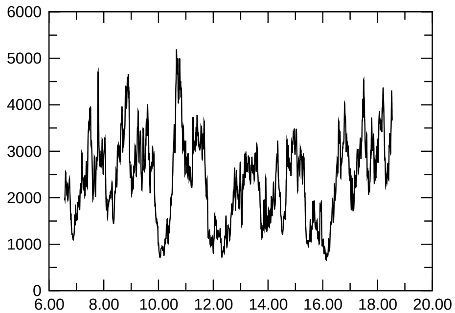
e065p08t1.75r110000m1p4mvbcFD E_{\text{magn}}
