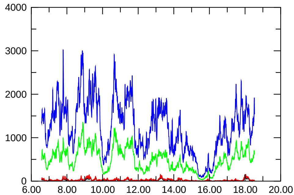
E_{\text{magn,dip.}}
