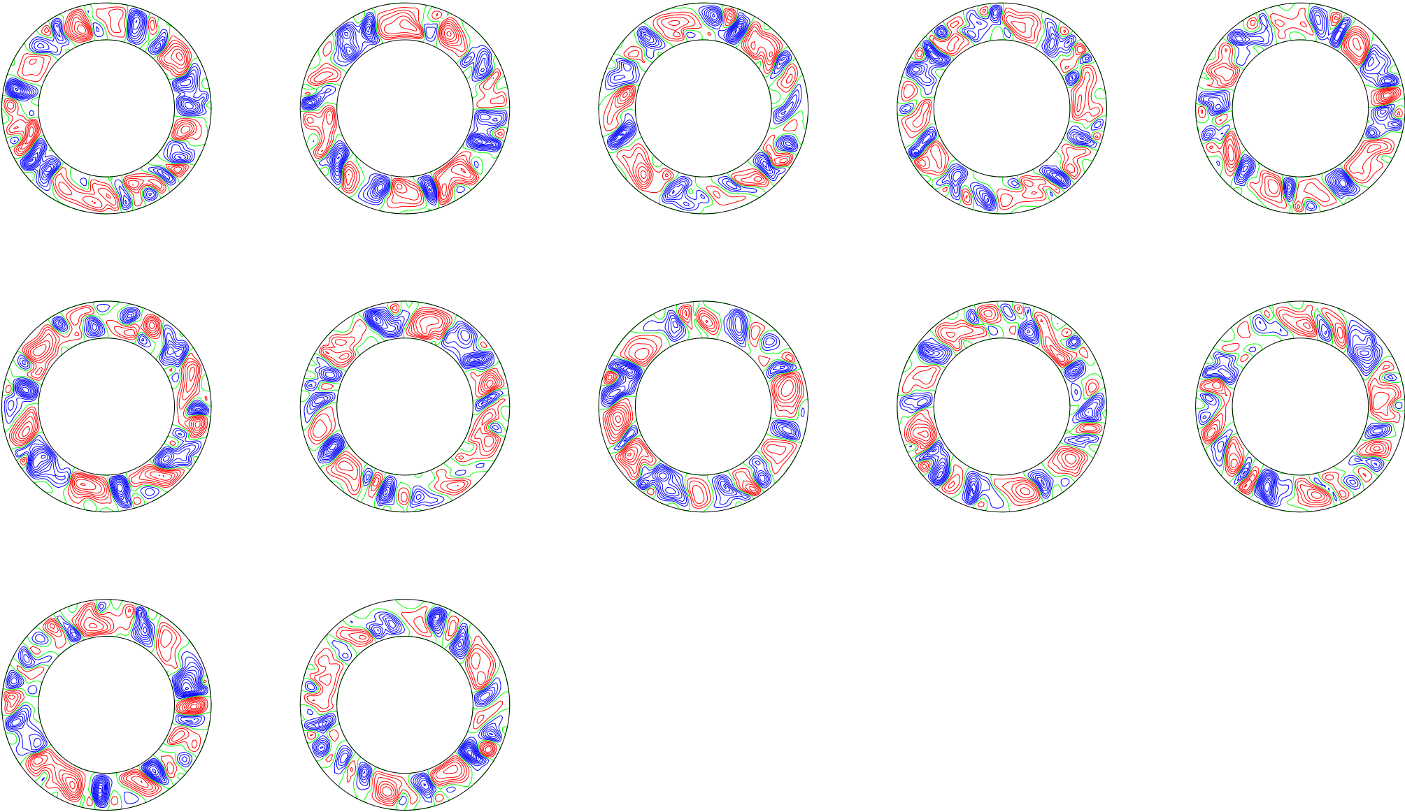
poloidal streamlines, (t[i] dt[i] t[i+1]): 20.72009 ( 0.56 ) 26.8802
