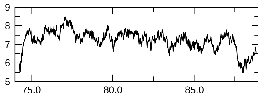
Btor(l=2,m=2) magn.
