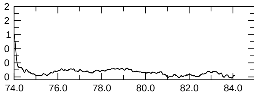
B_{\text{tor}}(l=2, m=2) magn.
