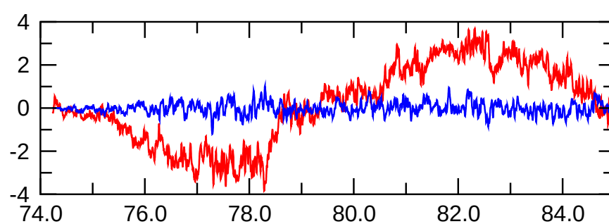
\text{pol}(m=0) magn.
