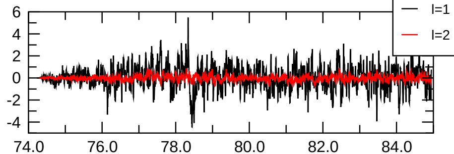
\text{pol}(m=2) magn.
