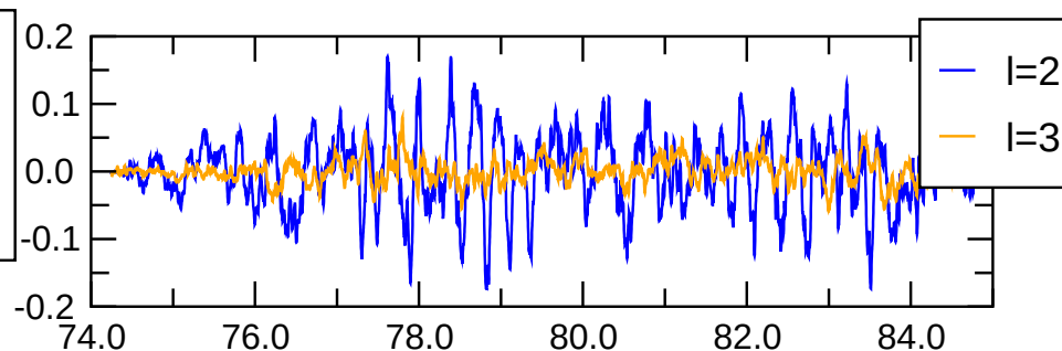
\text{pol}(m=0) magn.
