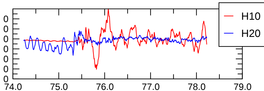
\text{pol}(m=0) magn.
