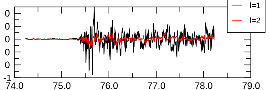
\text{pol}(m=2) magn.
