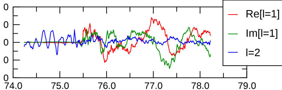
\text{pol}(m=0) magn.
