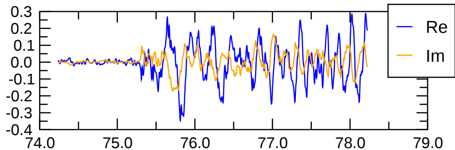
\text{pol}(m=1) magn.
