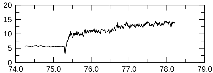
B\text{tor}(l=2, m=2) magn.
