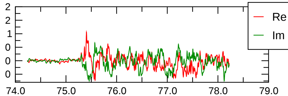
\text{tor}(m=0) magn.
