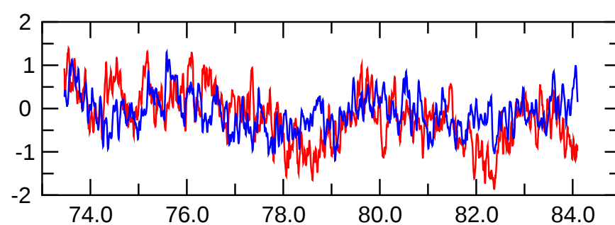
\text{pol}(m=0) magn.
