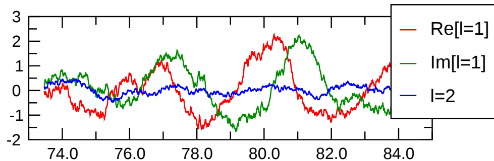
\text{pol}(m=1) magn.
