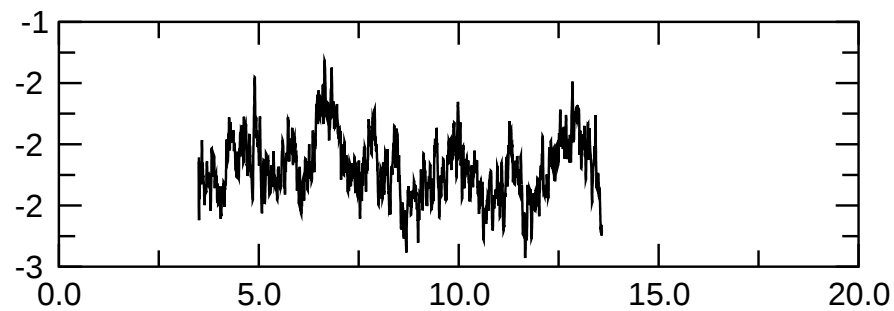
Btor(l=2,m=2) magn.
