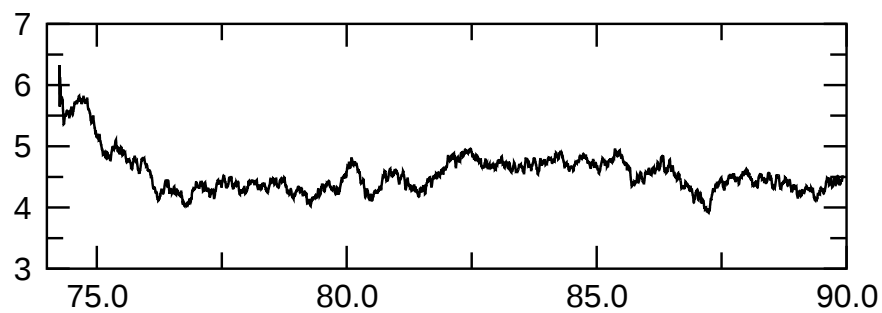
Btor(l=2,m=2) magn.
