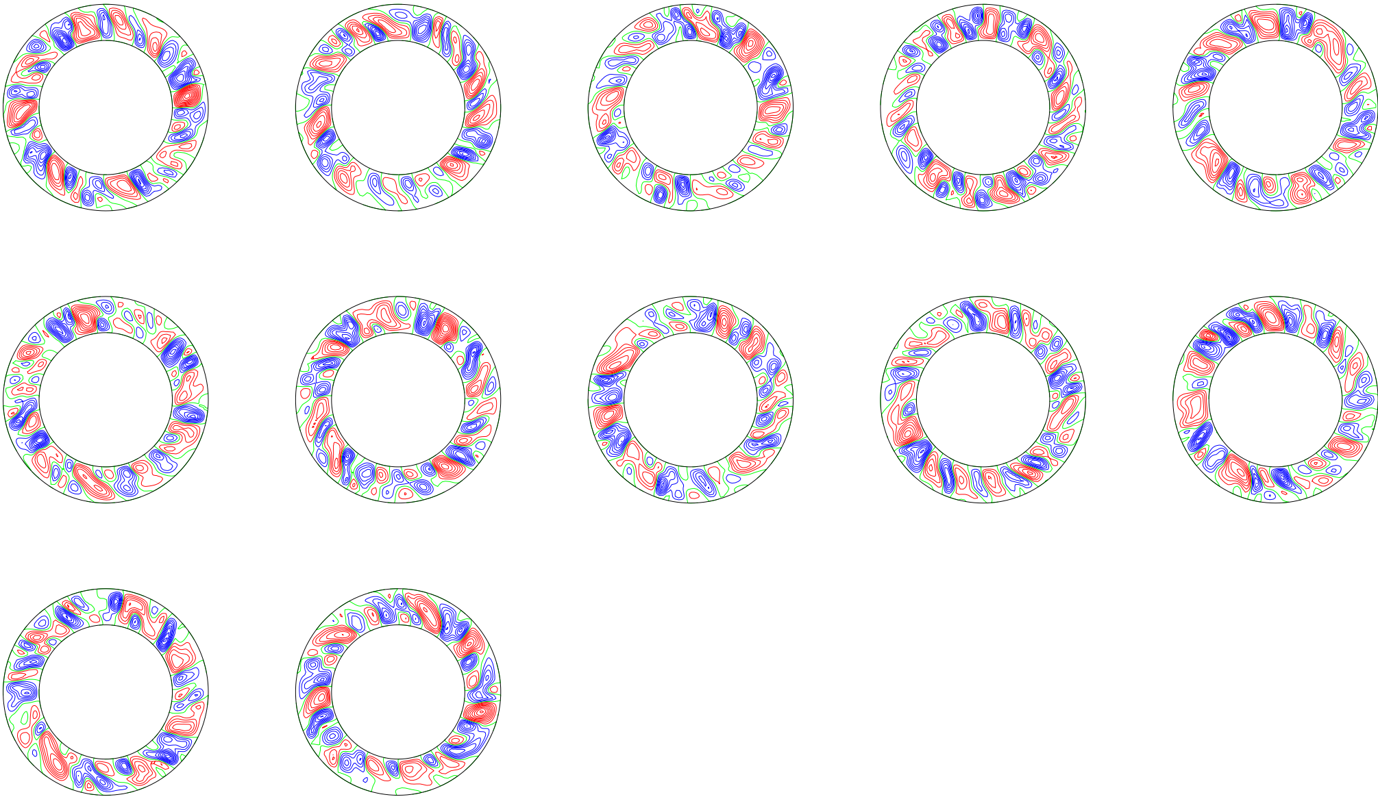
poloidal streamlines, (t[i] dt[i] t[i+1]): 72.4287 ( 0.028 ) 72.73681
