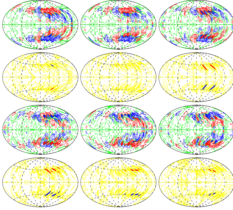
Figure 1: Half a period of oscillation in the case \eta = 0.65 , P = 1 , \tau = 2000 , R_e = 150000 , P_m = 4 , \beta = 1.5 with stress-free velocity boundary condition at r = r_o and no-slip at r = r_i . The odd rows show contour lines of B_r at r = 1 and the even rows show contour lines of -\frac{\partial g}{\partial \theta} at r = 0.9 . The time interval between the snapshots is 0.0112.
