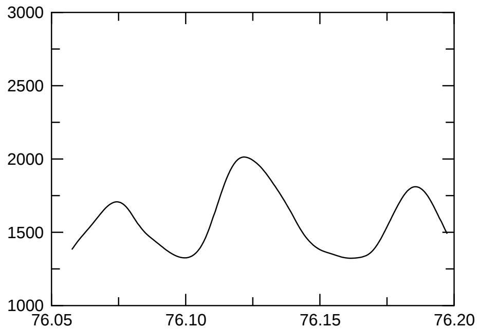
e065p1t2r150000m1p4mvbcFDsolrot1.5 E_{\text{magn}}
