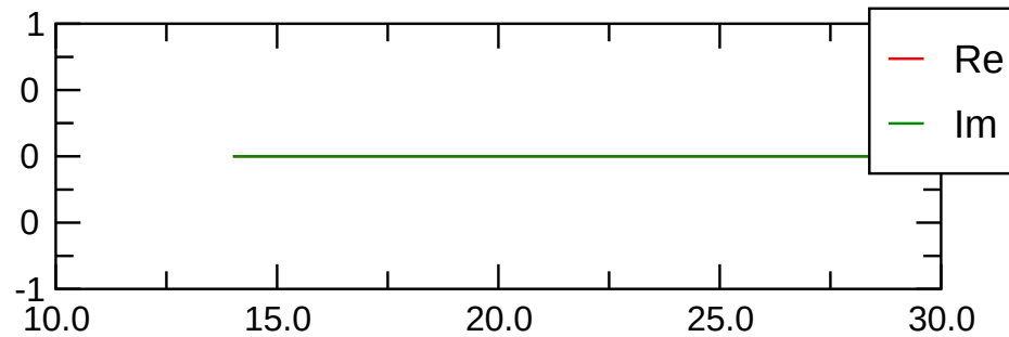
tor(m=0) magn.
