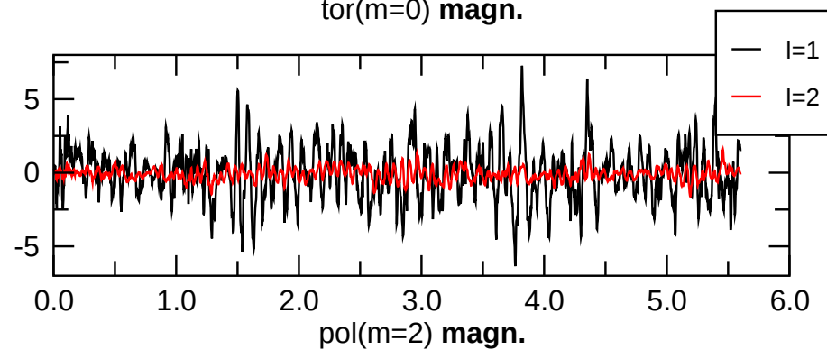
\text{tor}(m=0) magn.
