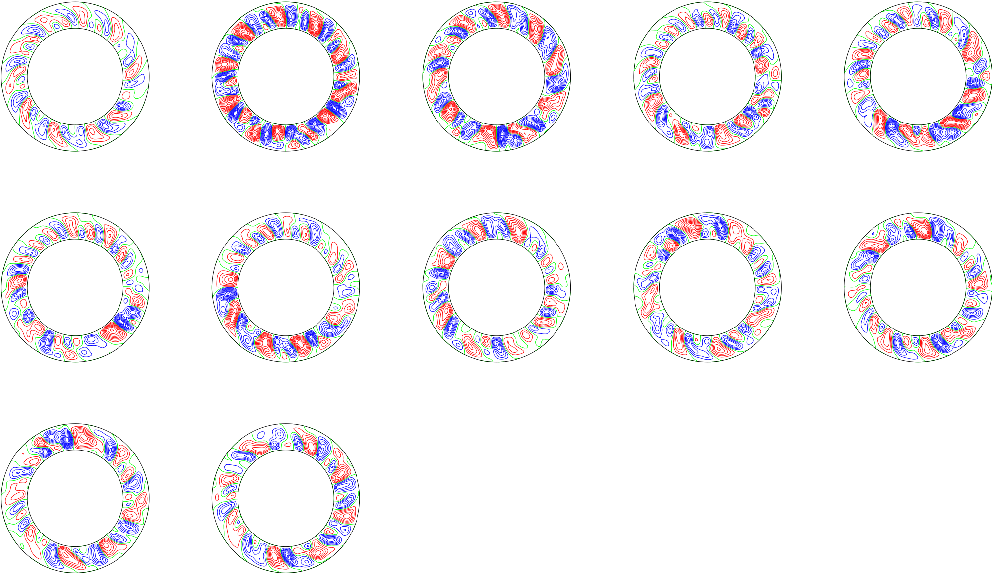
poloidal streamlines, (t[i] dt[i] t[i+1]): 0 ( 0.032 ) 0.352088
