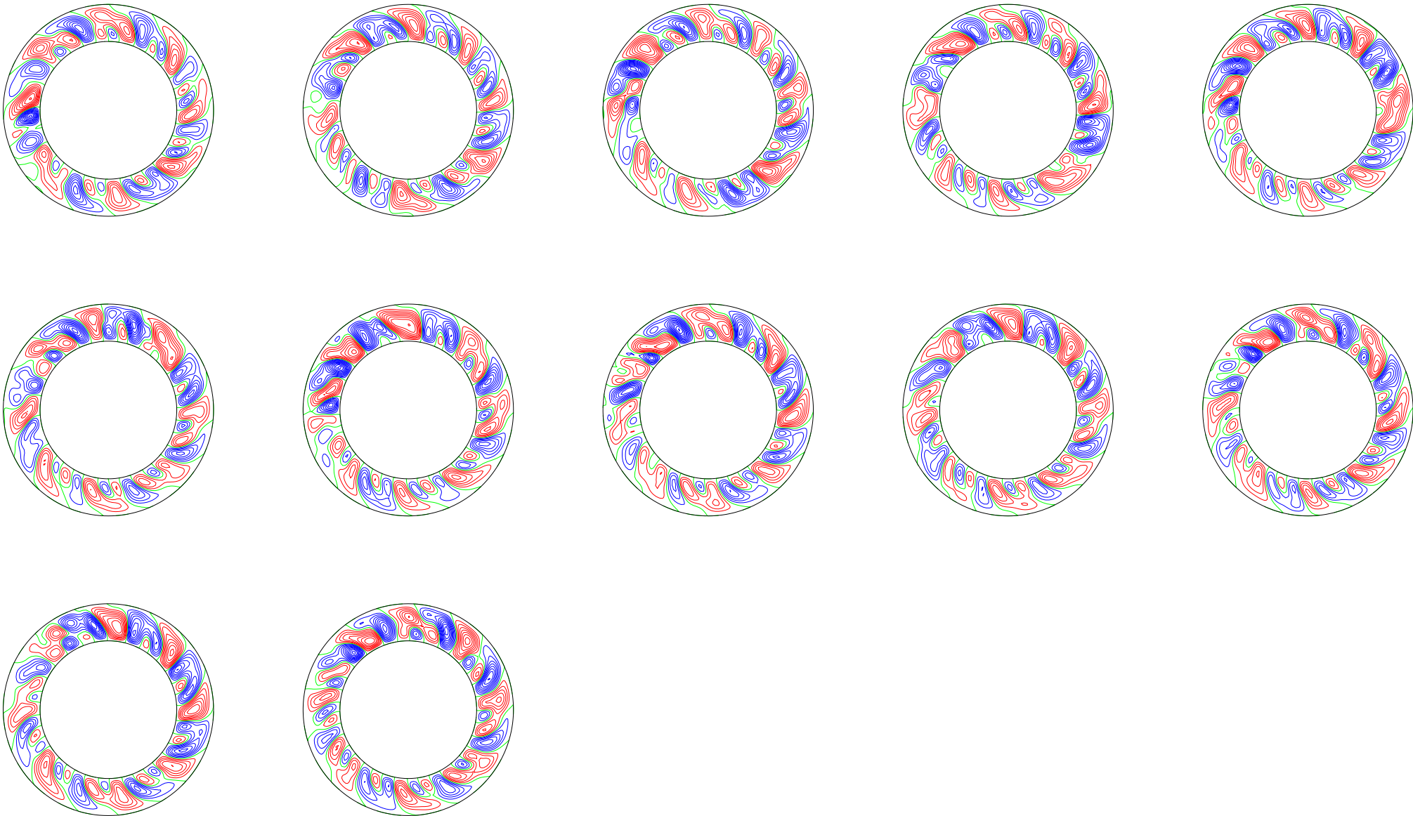
poloidal streamlines, (t[i] dt[i] t[i+1]): 1.856464 ( 0.032 ) 2.208552
