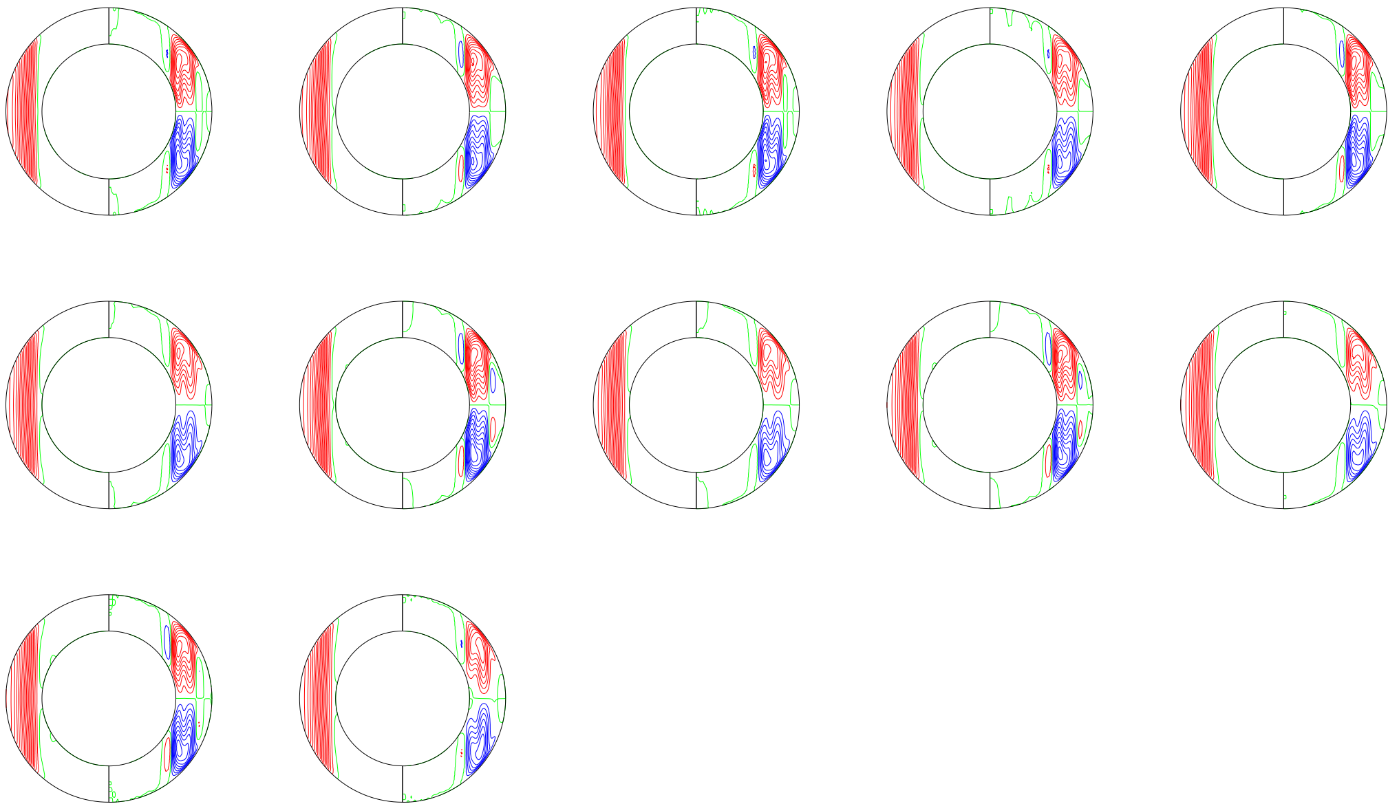
Uphi & merid strlines (merid. cut), (t[i] dt[i] t[i+1]): 0.704176 ( 0.032 ) 1.056264
