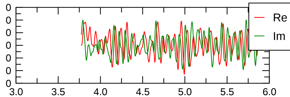
Btor( l=1, m=1 ) magn.
