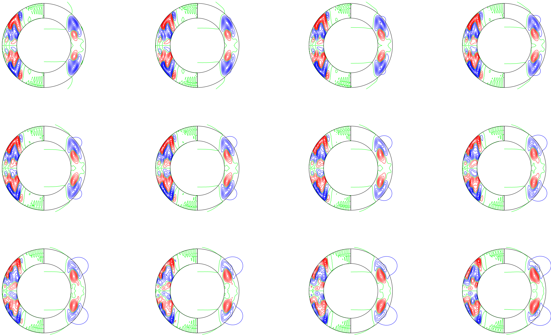
Bphi; mer. fieldlines, (t[i] dt[i] t[i+1]): 77.30453 ( 0.00256 ) 77.3328
