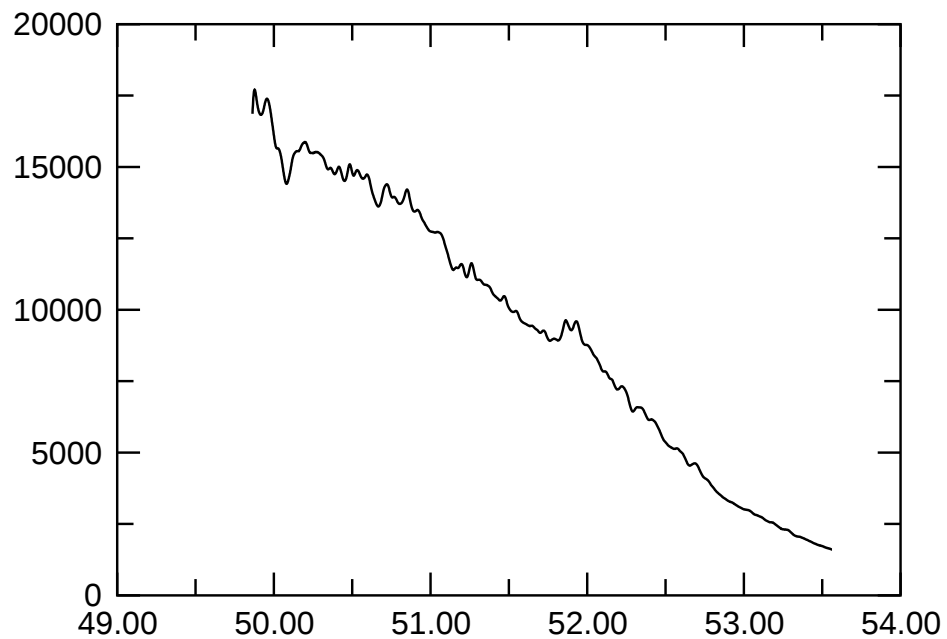
e065p1.2t2r100000m1p5.4mvbcMD E_{\text{magn}}
