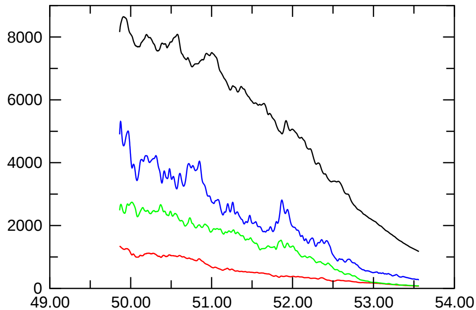
E_{\text{magn,dip.}}
