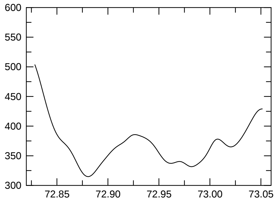
e065p1.2t2r120000m1p4.5mvbcFDsol01 E_{\text{magn}}
