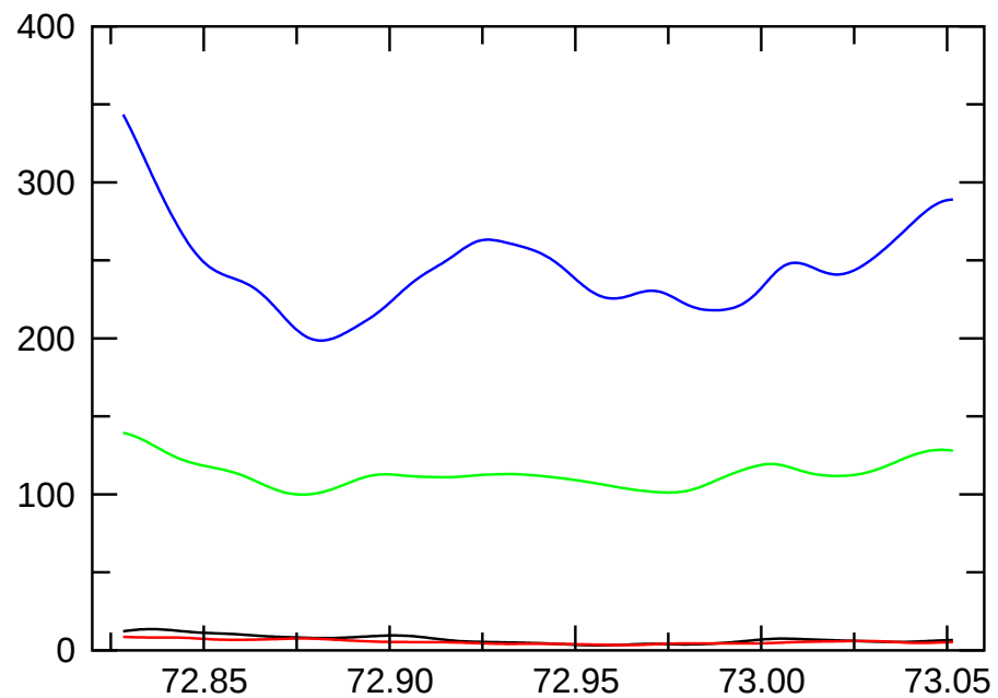
E_{\text{magn,dip.}}
