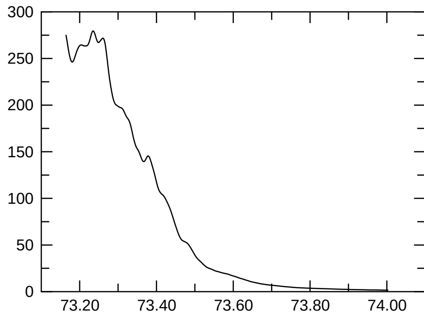
e065p1.2t2r120000m1p4.5mvbcFDsol2 E_{\text{magn}}
