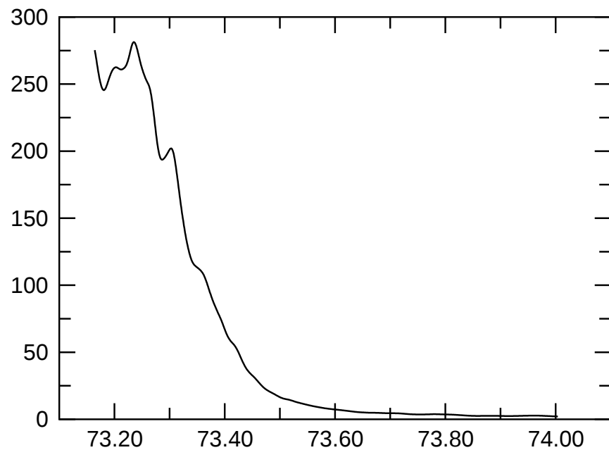
e065p1.2t2r120000m1p4.5mvbcFDsol5 E_{\text{magn}}
