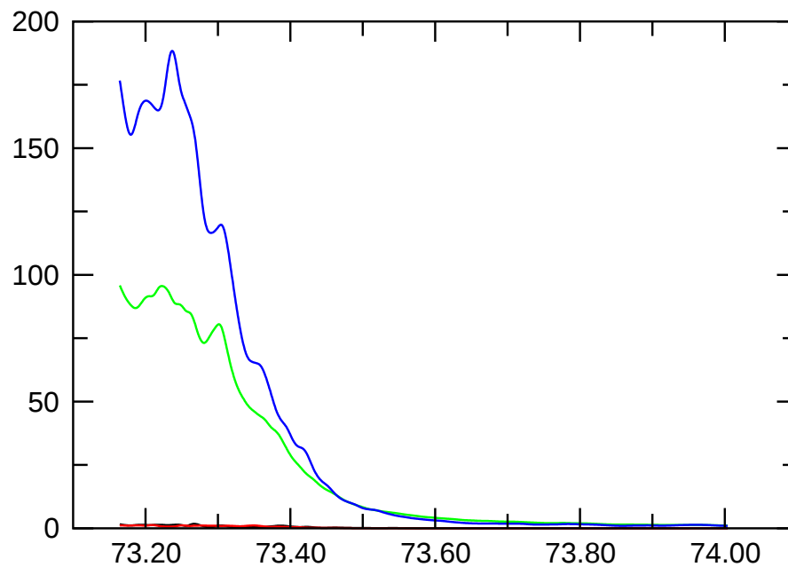
E_{\text{magn,dip.}}
