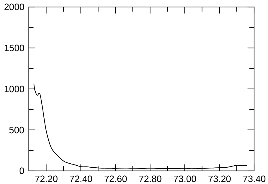
e065p1.2t2r120000m1p4.5mvbcSolFD E_{\text{magn}}
