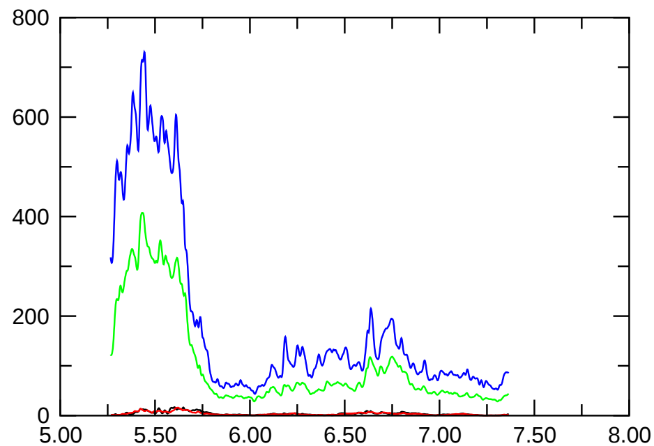
E_{\text{magn,dip.}}
