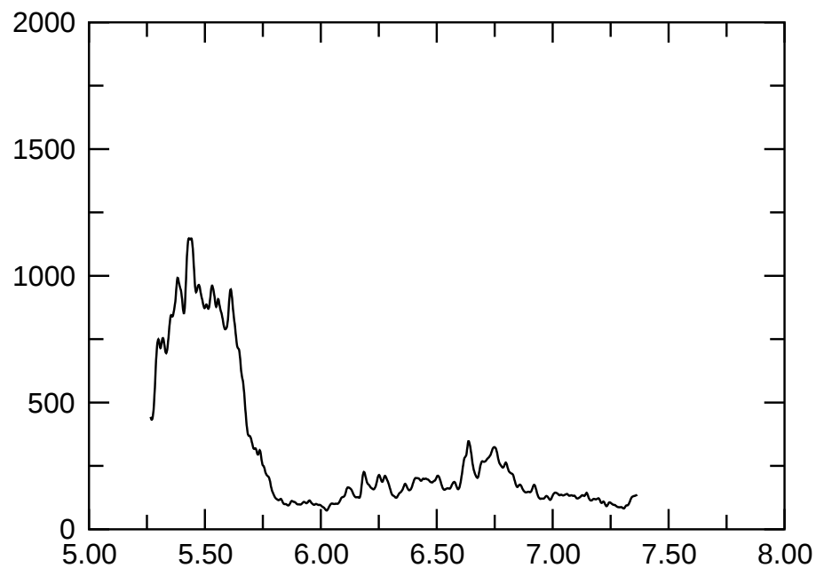
e065p1t1.75r120000m1p4mvbcFDsl1 E_{\text{magn}}
