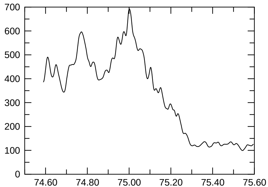
e065p1t2.5r150000m1p4mvbcFDsolrot1 E_{\text{magn}}
