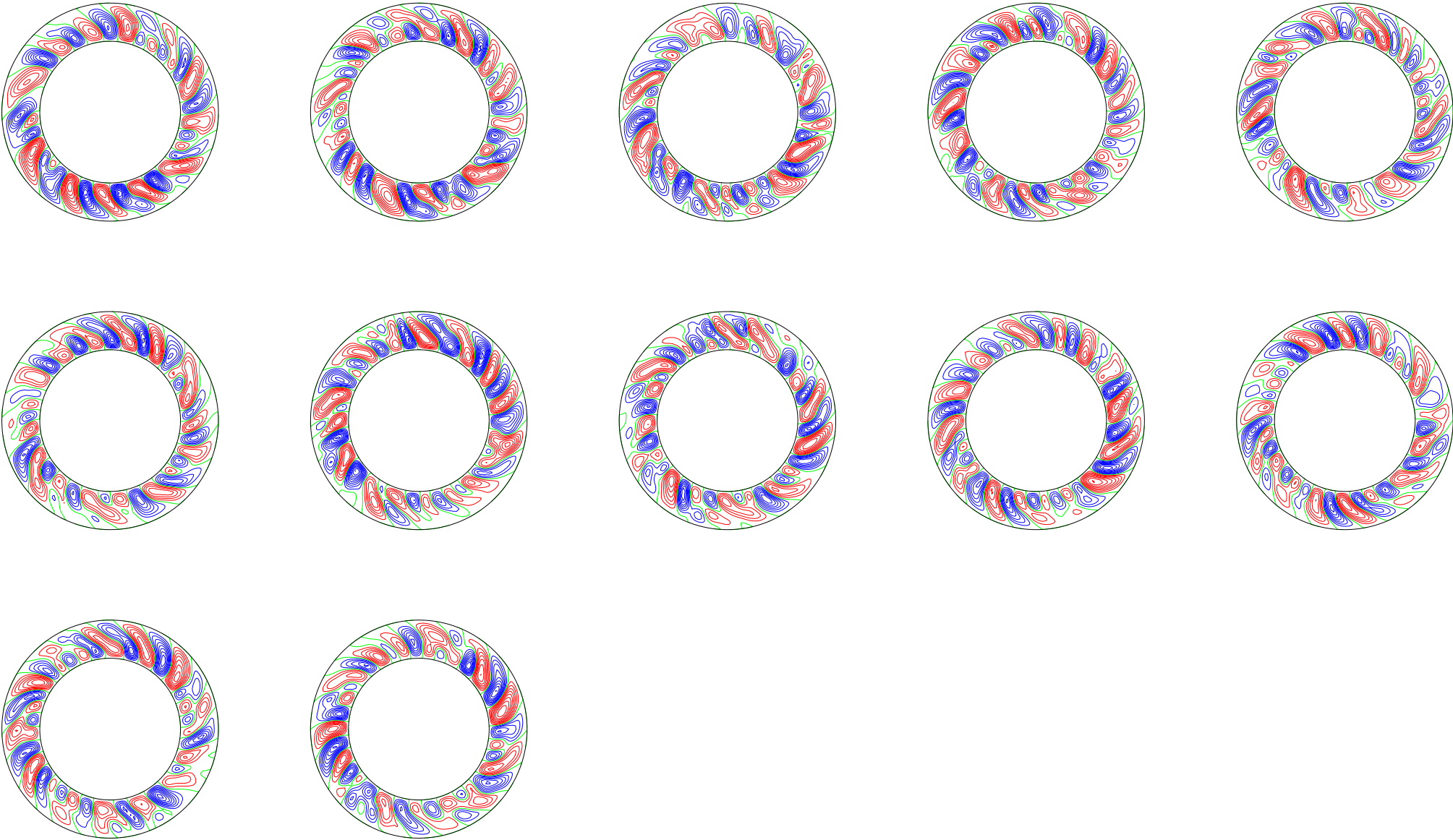
poloidal streamlines, (t[i] dt[i] t[i+1]): 75.05743 ( 0.14 ) 76.59754
