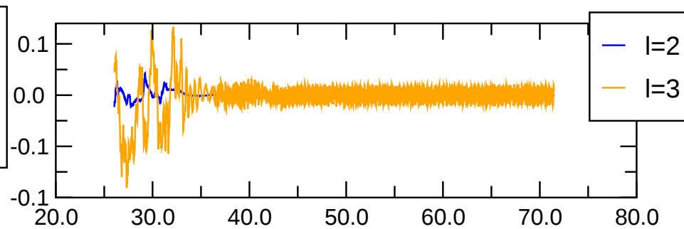
\text{pol}(m=0) magn.
