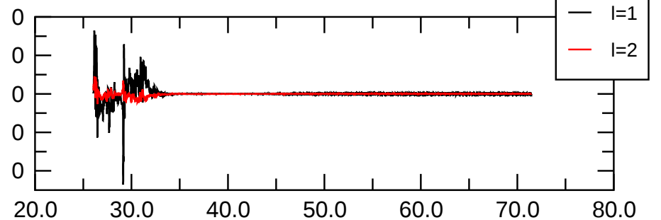
\text{pol}(m=2) magn.
