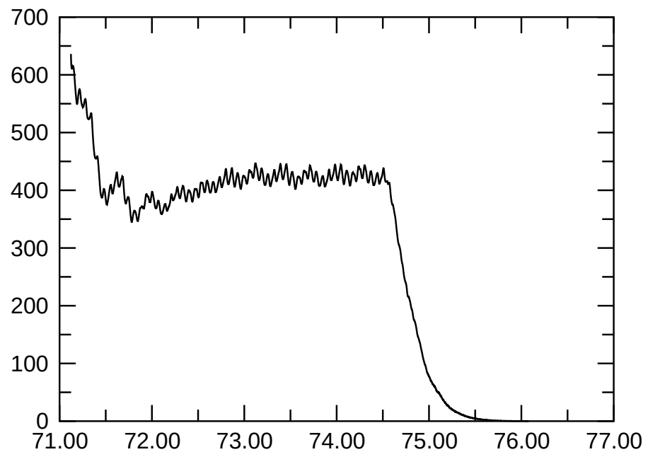
e065p1t2r100000m1p4mvbcFDsolrot1 E_{\text{magn}}
