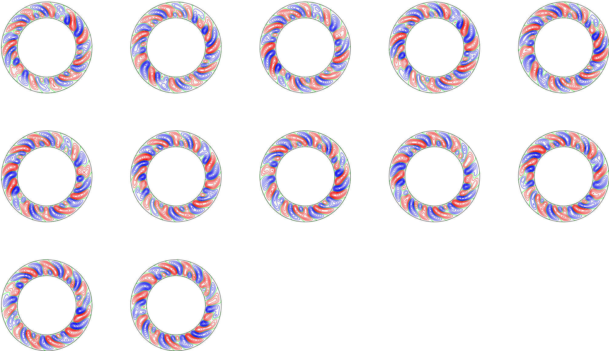
poloidal streamlines, (t[i] dt[i] t[i+1]): 74.42002 ( 0.021 ) 74.65113
