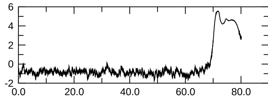
Btor(l=2,m=2) magn.
