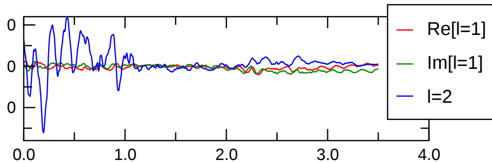
H10, H20 at r=r_i+1, (\text{magn})
