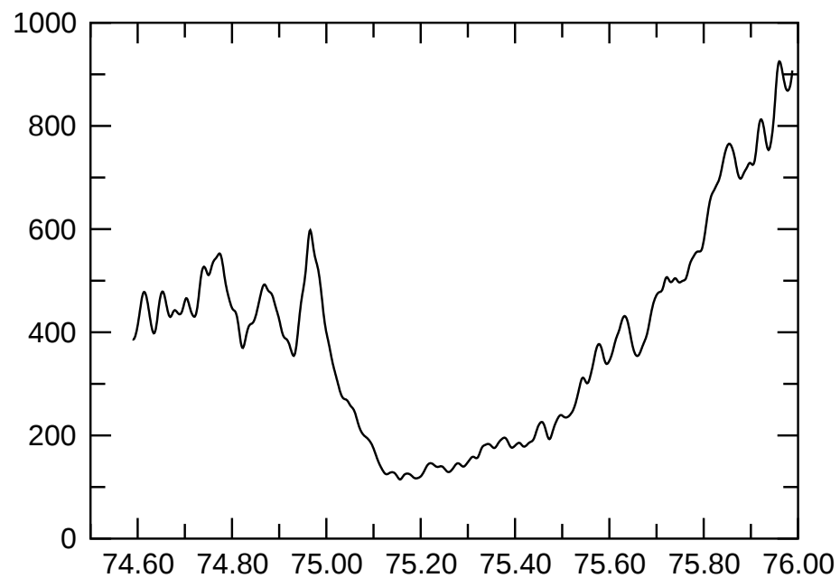
e065p1t2r120000m1p4mvbcFDsolrot08 E_{\text{magn}}
