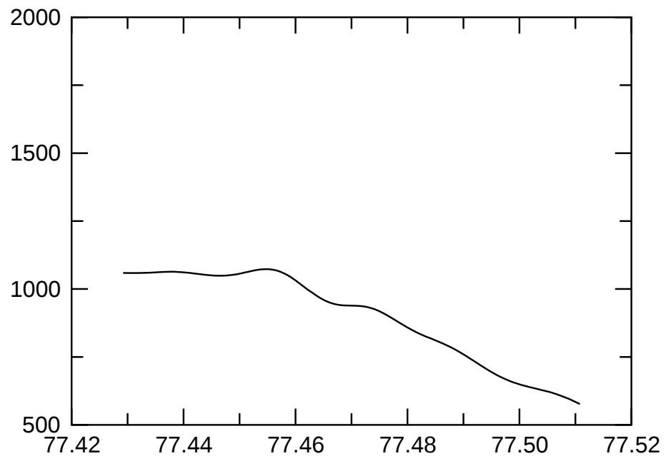
e065p1t2r120000m1p4mvbcFDsolrot1.5 E_{\text{magn}}
