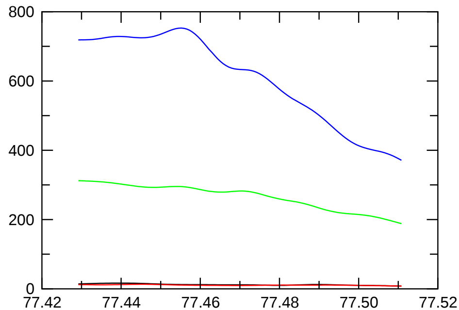
E_{\text{magn,dip.}}
