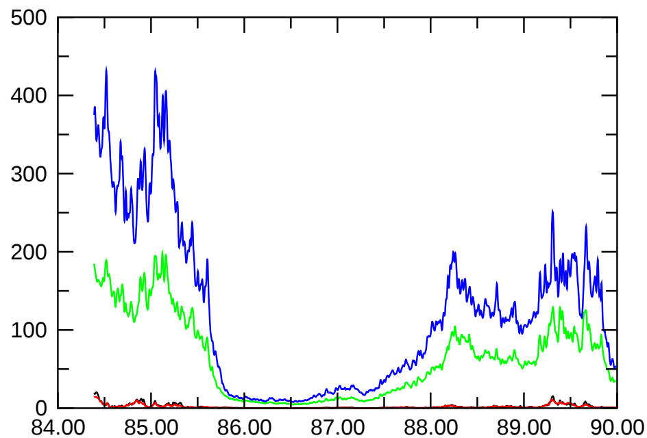
E_{\text{magn,dip.}}
