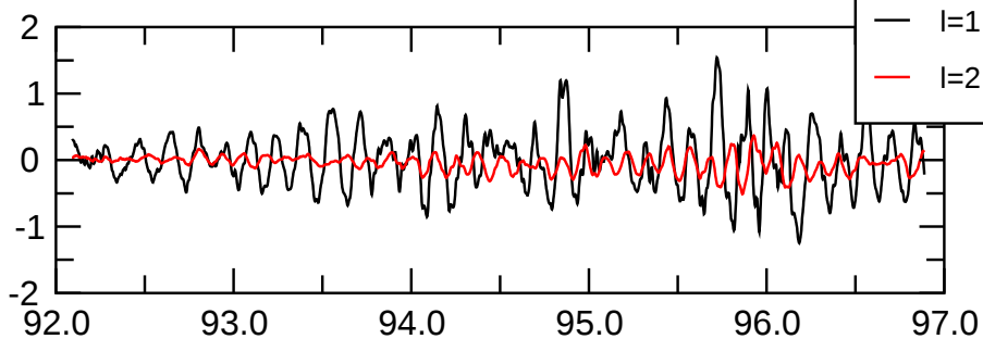
\text{pol}(m=2) magn.
