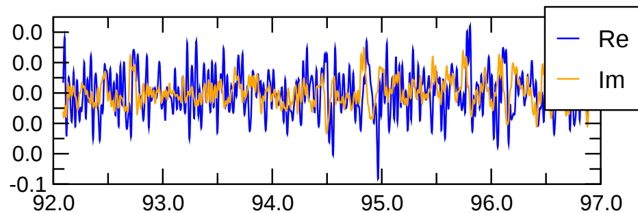
\text{pol}(m=1) magn.
