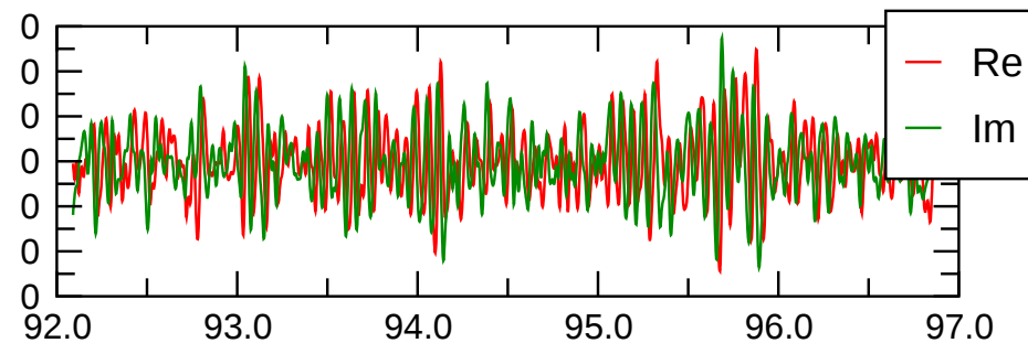
\text{tor}(m=0) magn.
