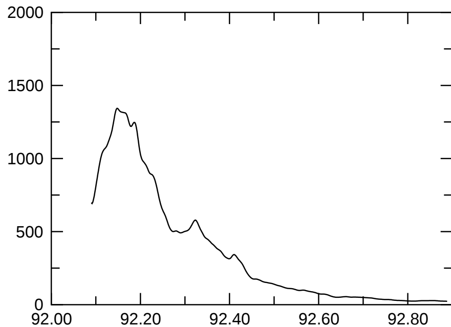
e065p1t2r130000m1p3.5mvbcFDsl08pc E_{\text{magn}}
