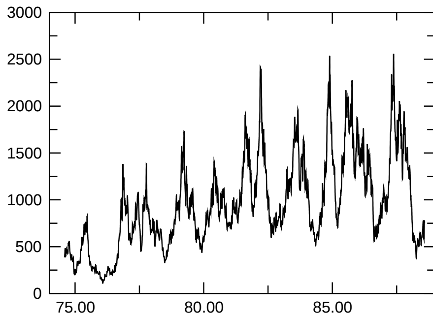
e065p1t2r130000m1p4mvbcFDsolrot08 E_{\text{magn}}
