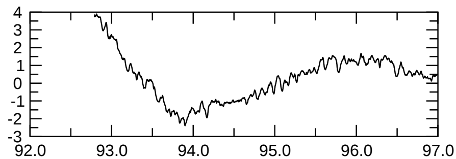
B\text{tor}(l=2, m=2) magn.
