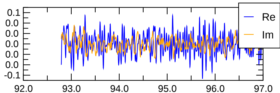
\text{pol}(m=1) magn.
