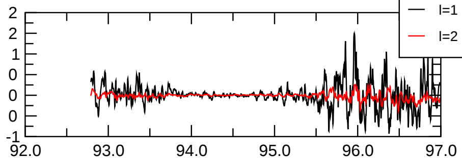
\text{pol}(m=2) magn.
