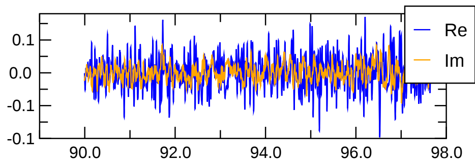
\text{pol}(m=1) magn.
