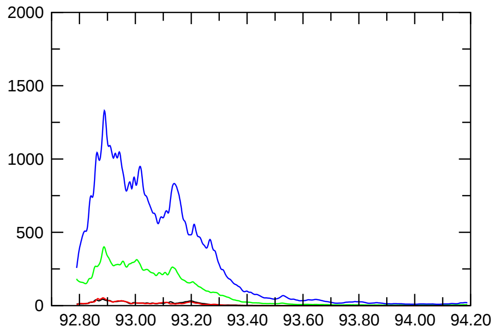
E_{\text{magn,dip.}}
