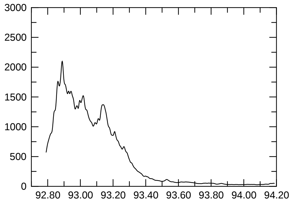
e065p1t2r140000m1p3.5mvbcFDsl1pc E_{\text{magn}}
