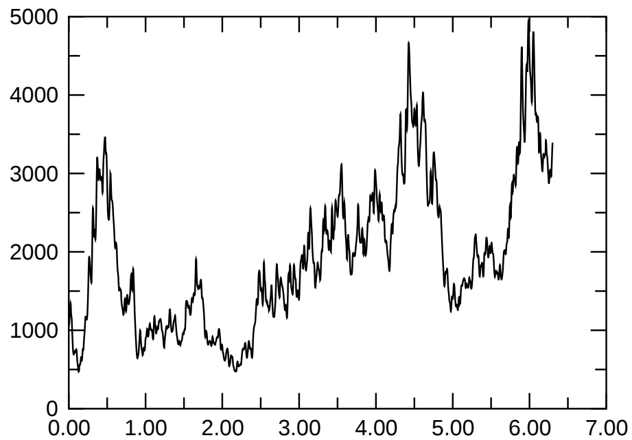
e065p1t2r140000m1p4mvbcFDsl05 E_{\text{magn}}
