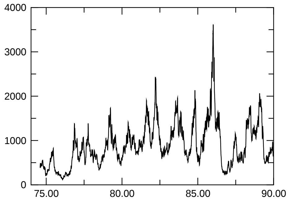
e065p1t2r140000m1p4mvbcFDsolrot1 E_{\text{magn}}
