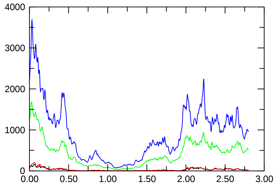
E_{\text{magn,dip.}}
